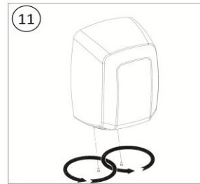
11 Screw the cover fixing screws (x2) Your dryer is now ready to be used on a Plug-in base
