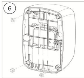
6 Remove the silent blocks from the back of the unit (x4)
