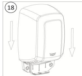
18 Mount the dryer over the Plug-in base with a from top to down movement
